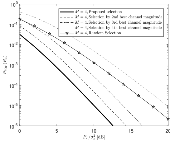
Fig. 29. SOP with different types of interfering RRH selection schemes.
