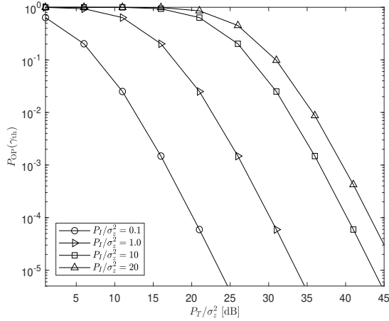
Fig. 21. Impact of interference power, P_I , on the outage probability.
