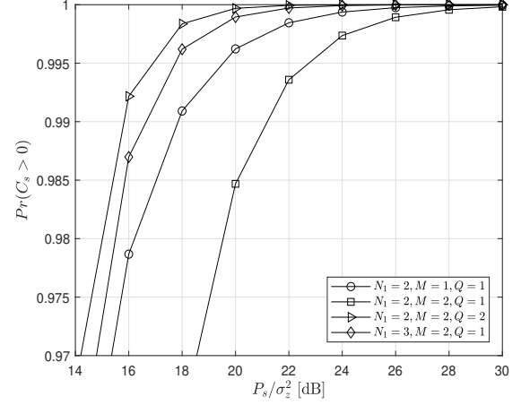
Fig. 25. Performance analysis: Probability of non-zero achievable secrecy rate.
