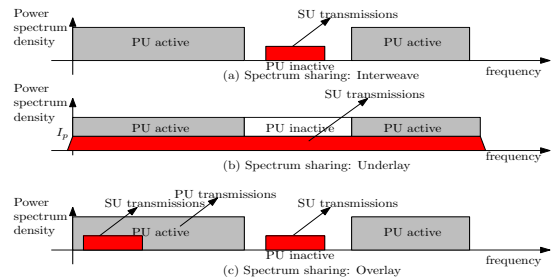
Fig. 15. Three different types of spectrum sharing.
