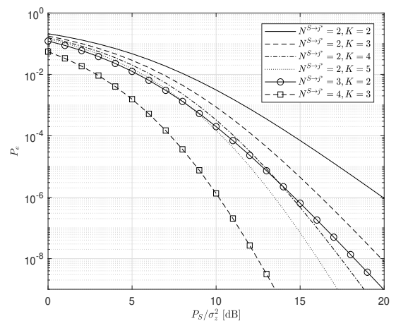
Fig. 11. ASER for various values of N^{S \rightarrow j^*} and K .
