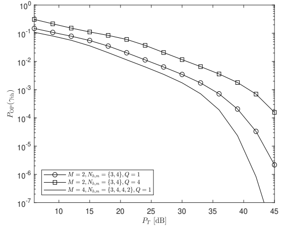
Fig. 27. Outage probability of the secondary network of dCDD-based spectrum sharing system.
