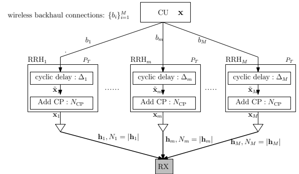
Fig. 8. Illustration of the under-populated dCDD-based CP-SC system, composed by one CU, M RRHs, and one RX.
