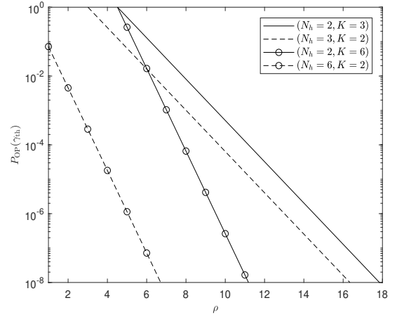
Fig. 7. Outage probability in terms of N_h and the number of users K . We use a fixed 1 dB threshold for \gamma_{th} .
