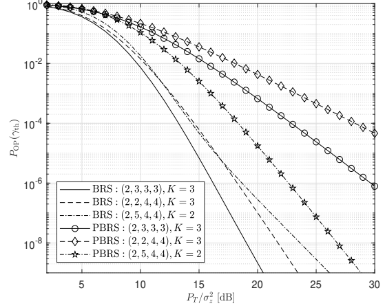
Fig. 17. Outage probability for various parameters. Two different relay selections are considered for comparisons. Elements of (N_1, N_2, N_3, N_4) respectively denote the number of multipath elements of \mathbf{h}^{S \rightarrow j} , \mathbf{h}^{j \rightarrow \text{D}} , \mathbf{g}^{S \rightarrow \text{PU}} , and \mathbf{f}^{j \rightarrow \text{PU}} .
