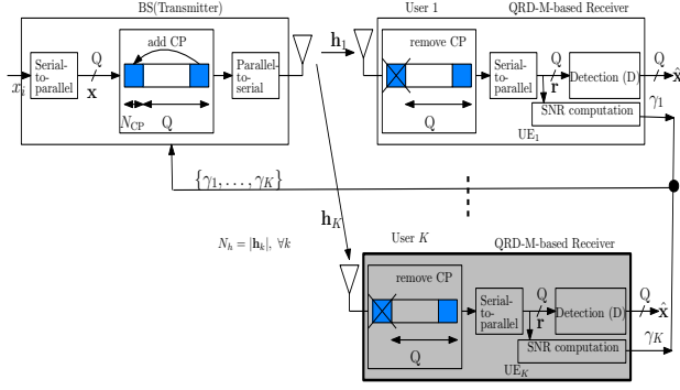
Fig. 6. CP-SC with opportunistic user scheduling. We assume that there are K users in the system. A highlighted user is selected for data transmissions.
