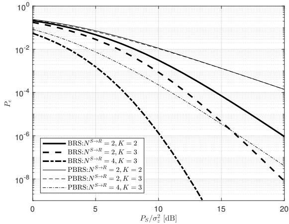
Fig. 12. ASER comparison of the CP-SC-based relaying systems with BRS and PBRs for various values of N^{S \rightarrow R} , R = \forall R_j and K .
