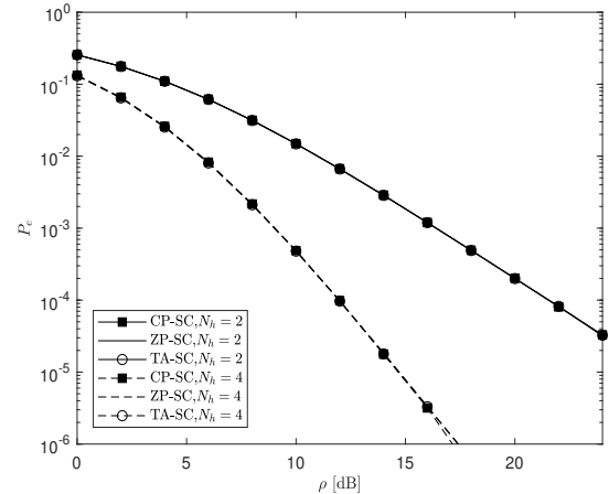
Fig. 5. ASER of CP-SC, TA-SC, and ZP-SC transmissions. QRD-M is employed at the receivers.
