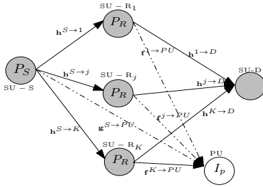
Fig. 16. Illustration of the CP-SC spectrum sharing system with the decode-and-forward (DF) relaying protocol. K SU-relays, \{\text{SU-R}_j\}_{k=1}^K , and PU are assumed in the system. The SU network is composed by the SU-S, SU-relays, and SU-destination (SU-D).
