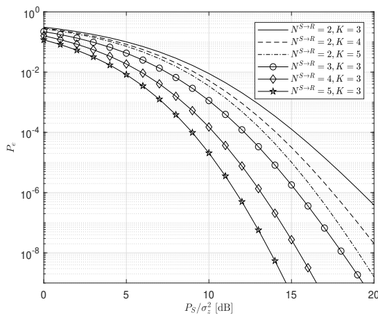
Fig. 14. ASER for various values of N^{S \rightarrow R} and K .
