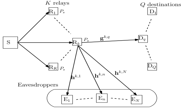
Fig. 23. Illustration of the cooperative PLS system with CP-SC transmissions.
