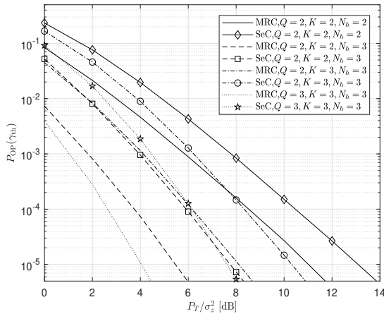
Fig. 19. Outage probability of the spectrum sharing system for various parameters. K PU receivers are assumed in the system.
