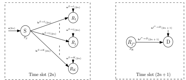
Fig. 10. AF-based CP-SC relaying system with best relay selection (BRS).
