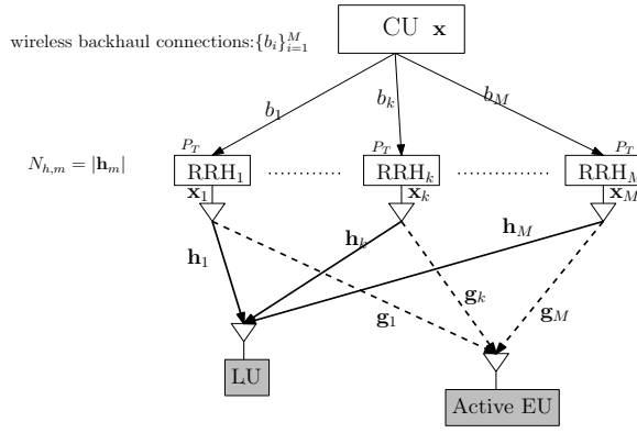
Fig. 28. Illustration of the dCDD-based cooperative system with PLS in the presence of one active EU.
