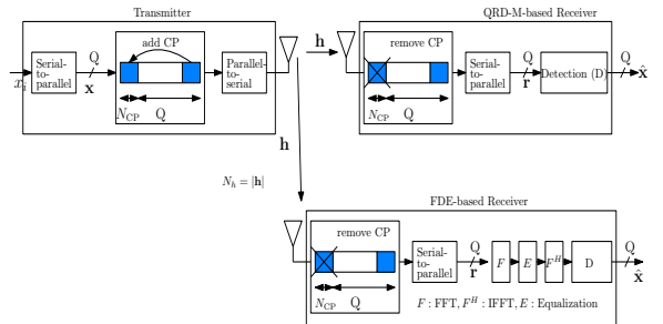
Fig. 2. Block diagram of the wireless communication system employing CP-SC transmissions. QR decomposition-M (QRD-M)-based and frequency domain equalizer (FDE)-based data detectors are respectively considered in two receivers.
