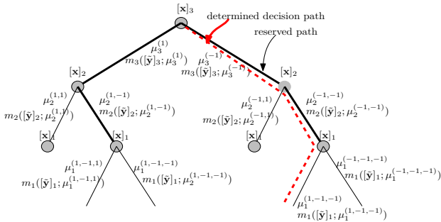
Fig. 3. One example of QRD-M-based data detection process.
