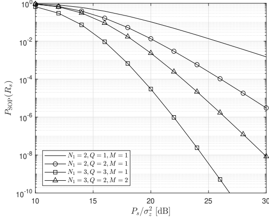
Fig. 24. Performance analysis: SOP.
