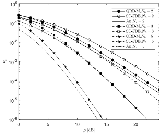
Fig. 4. ASER of CP-SC transmissions. In this simulation, N_h denotes the number of multipath of \mathbf{h} .
