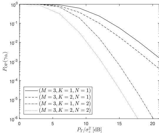
Fig. 9. Outage probability in terms of (M, K, N = \{N_m\}_{m=1}^M) .
