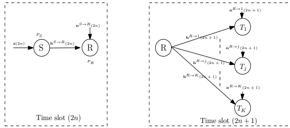
Fig. 13. AF-based CP-SC relaying system with opportunistic best terminal selection (BTS).
