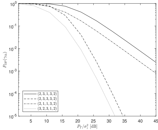
Fig. 22. The outage probability for various (M, N, N_h, N_f, N_g) s that specify system and channel parameters.
