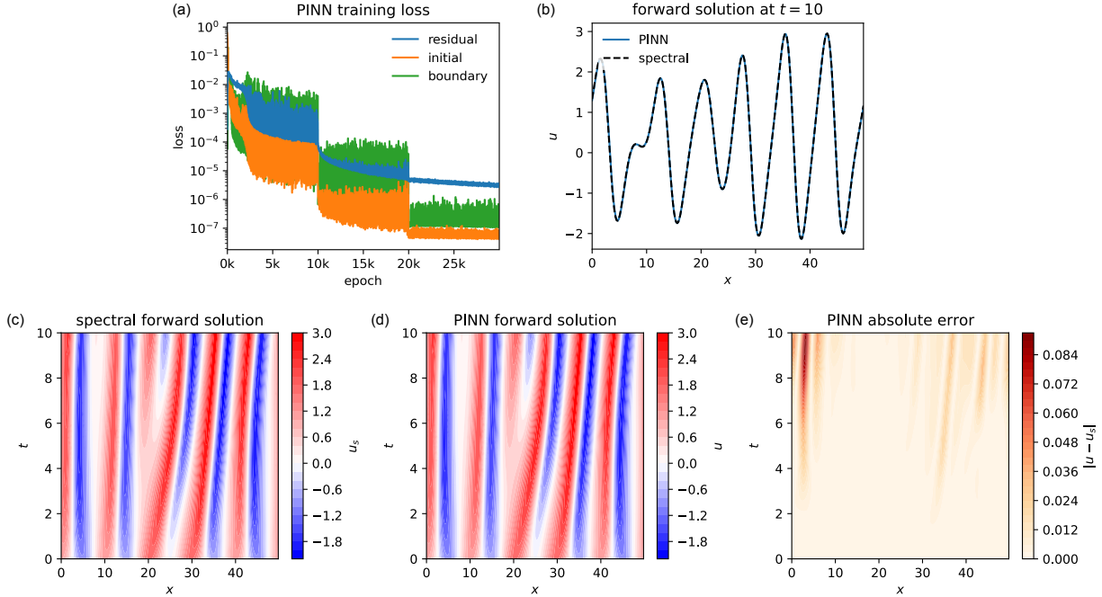
Figure 6 – Forward solution of the KS equation (32). (a) Convergence of the loss during training of the PINN solution. (b) Snapshots at final time of the trained PINN solution and a reference spectral solution. (c) Reference spectral solution u_s , (d) trained PINN solution u and (e) its local absolute error |u - u_s|
