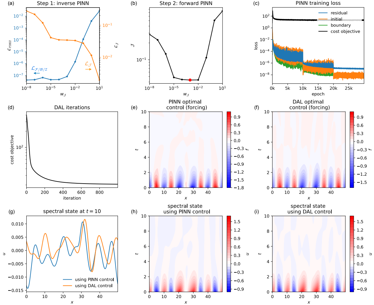
Figure 7 – Optimal solution of the KS control problem (34). (a) Components of the loss (20) obtained at the end of training of the PINN optimal control solution versus weight w_{\mathcal{J}} (step 1 of the line search strategy). (b) Cost objective estimate obtained by a separate PINN solution of the forward problem with fixed control from the PINN optimal solution versus w_{\mathcal{J}} (step 2 of the line search strategy). The best optimal control, obtained with w_{\mathcal{J}} = 10^{-3} , is shown by the red dot. (c) Convergence of the loss during training of the PINN optimal control solution (for w_{\mathcal{J}} = 10^{-3} ). (d) Convergence of the cost objective during DAL iterations. (e,f) Optimal control forces f^* obtained from the PINN (for w_{\mathcal{J}} = 10^{-3} ) and DAL frameworks. (g,h,i) Snapshots at final time and contour plots of two spectral solutions calculated using the optimal control forces f^* obtained from the PINN (for w_{\mathcal{J}} = 10^{-3} ) and DAL frameworks.
