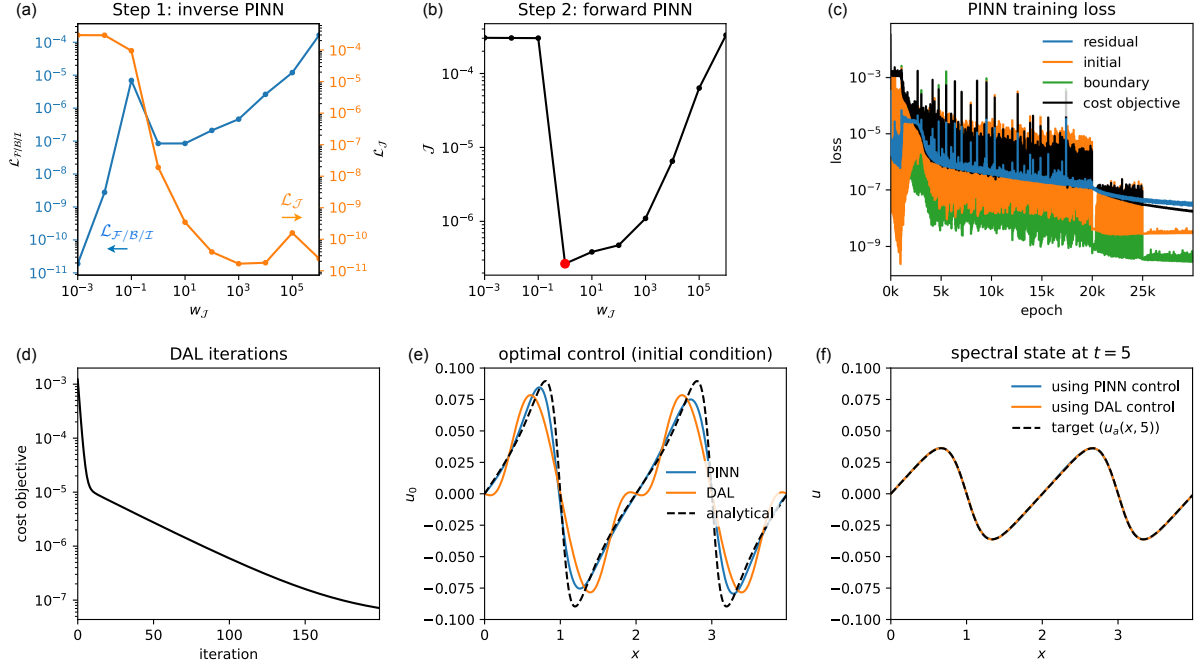
Figure 5 – Optimal solution of the Burgers control problem (30). (a) Components of the loss (20) obtained at the end of training of the PINN optimal control solution versus weight w_{\mathcal{J}} (step 1 of the line search strategy). (b) Cost objective estimate obtained by a separate PINN solution of the forward problem with fixed control from the PINN optimal solution versus w_{\mathcal{J}} (step 2 of the line search strategy). The best optimal control, obtained with w_{\mathcal{J}} = 1 , is shown by the red dot. (c) Convergence of the loss during training of the PINN optimal control solution (for w_{\mathcal{J}} = 1 ). (d) Convergence of the cost objective during DAL iterations. (e) Optimal initial condition u_0^* obtained using the PINN (for w_{\mathcal{J}} = 1 ) and DAL frameworks, compared with the initial state of the analytical solution. (f) Snapshots at final time of two spectral solutions calculated using the optimal initial conditions u_0^* from the PINN Convergence of the loss during training of the PINN optimal control solution (for w_{\mathcal{J}} = 1 ) and DAL frameworks, compared with the final state of the analytical solution.
