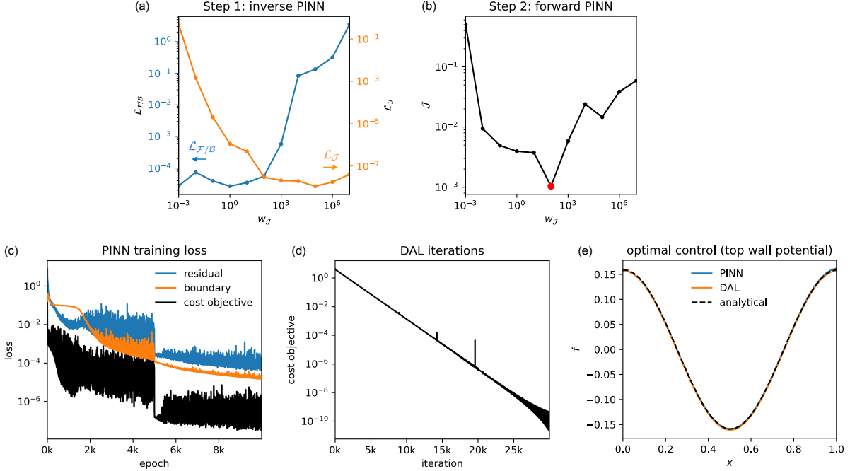
Figure 3 – Optimal solution of the Laplace control problem (25). (a) Components of the loss (20) obtained at the training of the PINN optimal control solution versus weight w_{\mathcal{J}} (step 1 of the line search strategy). (b) Cost objective estimate obtained by a separate PINN solution of the forward problem with fixed control from the PINN optimal solution versus w_{\mathcal{J}} (step 2 of the line search strategy). The best optimal control, obtained with w_{\mathcal{J}} = 100 , is shown by the red dot. (c) Convergence of the loss during training of the PINN optimal control solution (for w_{\mathcal{J}} = 100 ). (d) Convergence of the cost objective during DAL iterations. (e) Optimal top wall potential f^* obtained from the PINN (for w_{\mathcal{J}} = 100 ) and DAL frameworks, compared with the top wall potential f_a^* of the analytical solution.
