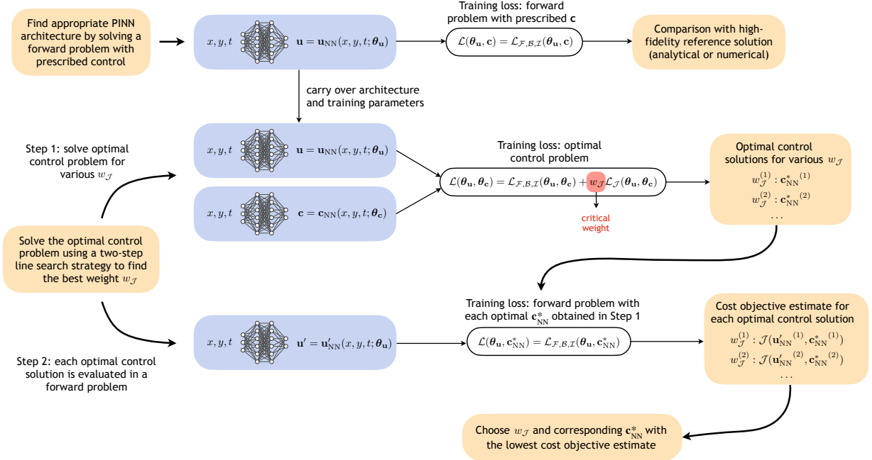
Figure 1 – Guidelines for obtaining a good optimal control solution using the PINN framework.
