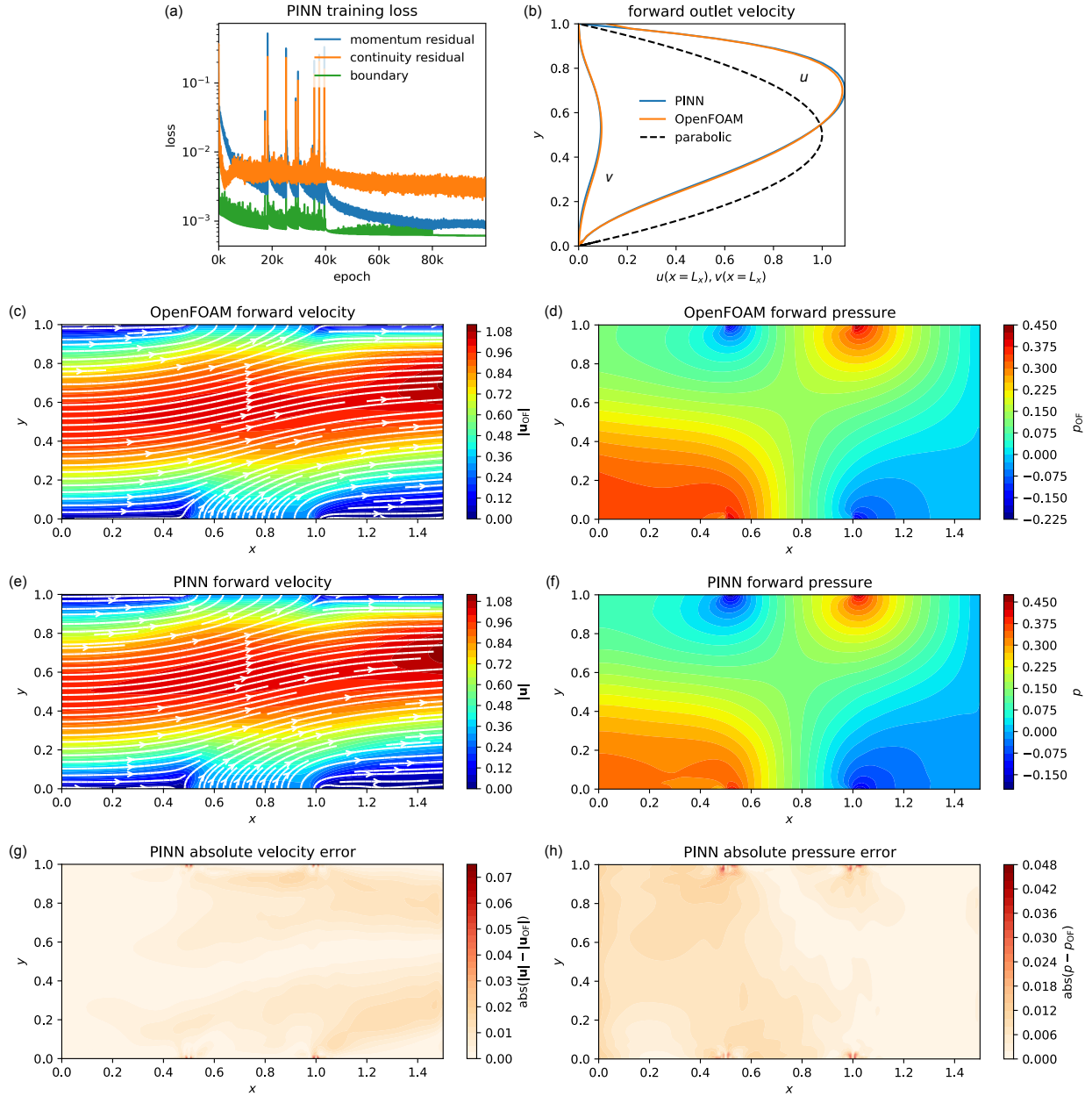
Figure 9 – Forward solution of the Navier-Stokes equation (36). (a) Convergence of the loss during training of the PINN solution. (b) Velocity profile at the outlet \Gamma_o of the trained PINN and the reference OpenFOAM solution. (c,e,g) Velocity magnitude and streamlines of the OpenFOAM and trained PINN solutions, and absolute error between them. (d,f,h) Pressure field of the OpenFOAM and trained PINN solutions.
