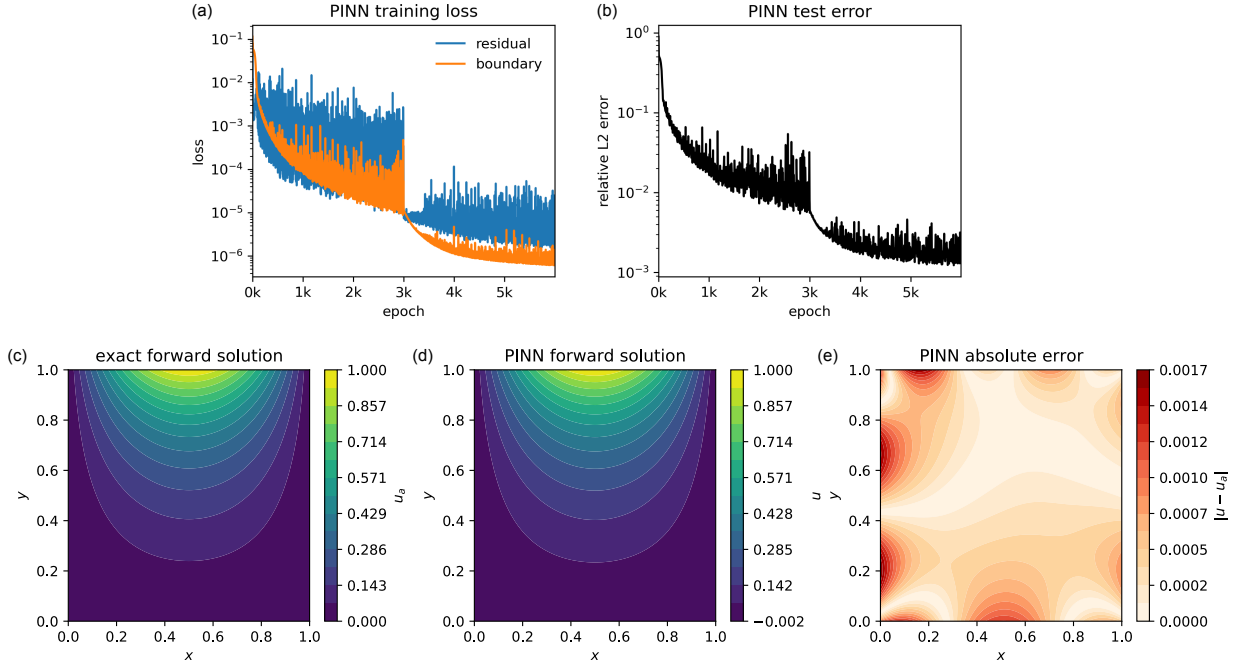
Figure 2 – Forward solution of the Laplace equation (21). (a,b) Convergence of the loss and relative L_2 test error during training of the PINN solution. (c) Analytical solution u_a , (d) trained PINN solution u and (e) its local absolute error |u - u_a| .
