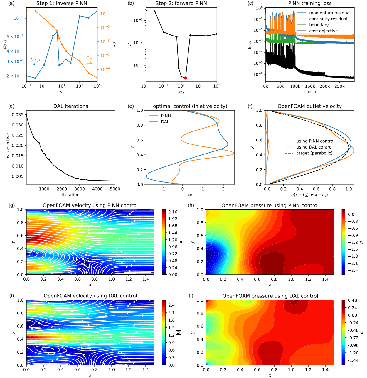
Figure 10 – Optimal solution of the Navier-Stokes control problem (39). (a) Components of the loss (20) obtained at the end of training of the PINN optimal control solution versus weight w_{\mathcal{J}} (step 1 of the line search strategy). (b) Cost objective estimate obtained by a separate PINN solution of the forward problem with fixed control from the PINN optimal solution versus w_{\mathcal{J}} (step 2 of the line search strategy). The best optimal control, obtained with w_{\mathcal{J}} = 30 , is shown by the red dot. (c) Convergence of the loss during training of the PINN optimal control solution (for w_{\mathcal{J}} = 30 ). (d) Convergence of the cost objective during DAL iterations. (e) Optimal inlet velocity profiles u_{in}^* obtained using the PINN (for w_{\mathcal{J}} = 30 ) and DAL frameworks. (f) Outlet velocity profiles of two forward OpenFOAM solutions calculated using the optimal inlet profiles u_{in}^* from the PINN (for w_{\mathcal{J}} = 30 ) and DAL frameworks, compared with the target parabolic profile. (f,g,h,i) Velocity magnitude, streamlines and pressure fields of the OpenFOAM solutions calculated using the optimal inlet profiles u_{in}^* from the PINN (for w_{\mathcal{J}} = 30 ) and DAL frameworks.
