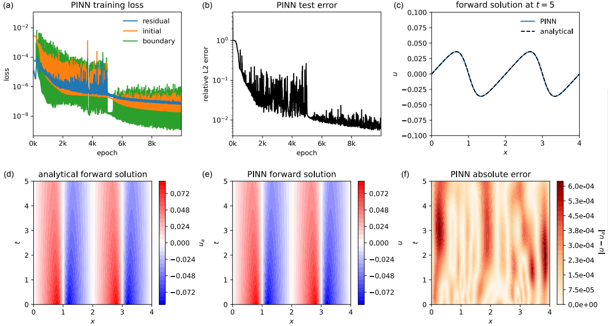
Figure 4 – Forward solution of the Burgers equation (28). (a,b) Convergence of the loss and relative L_2 test error during training of the PINN solution. (c) Snapshots at final time of the trained PINN and analytical solutions. (d) Analytical solution u_a , (e) trained PINN solution u and (f) its local absolute error |u - u_a| .
