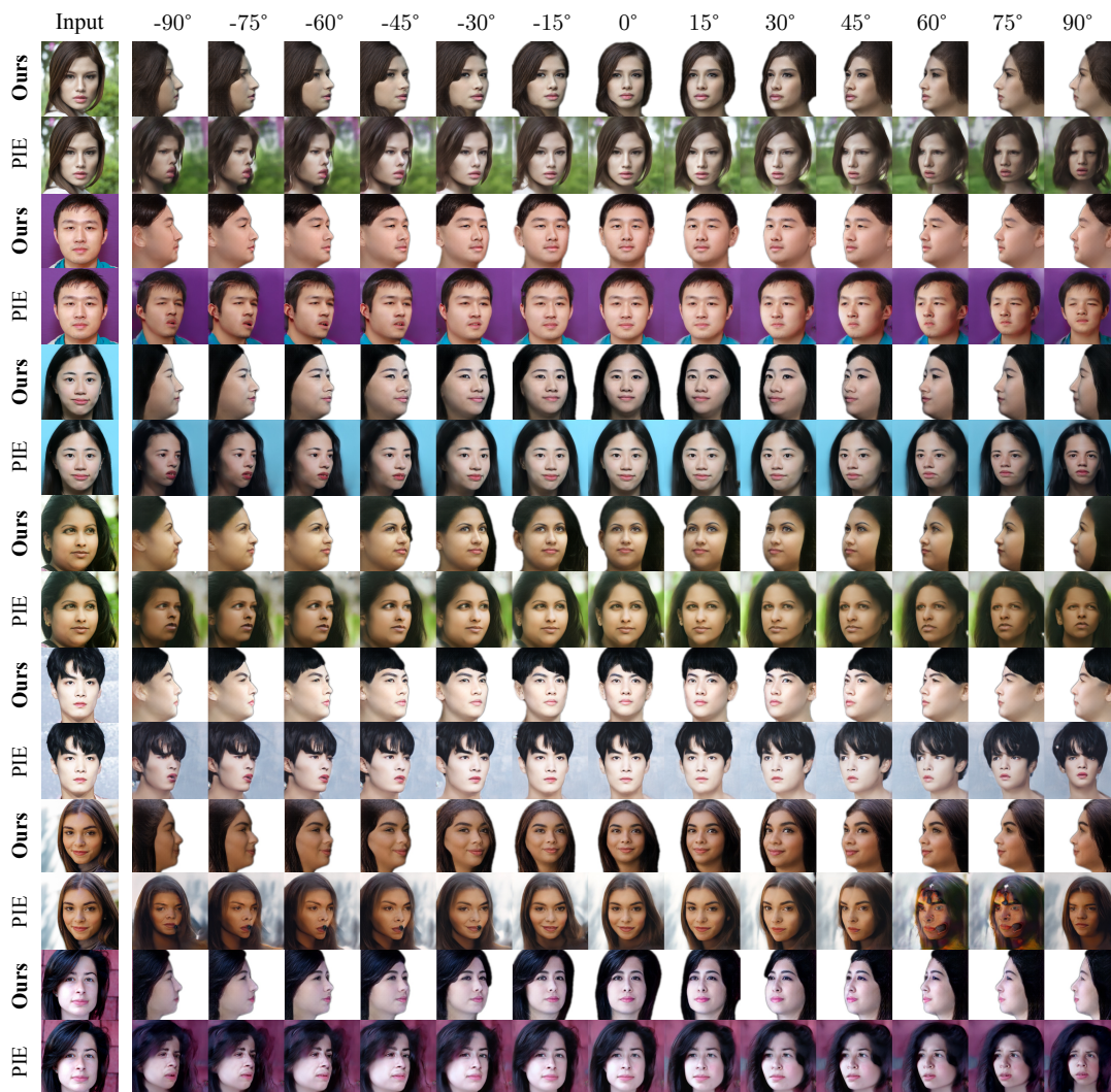
Figure 12: Pose manipulation results and comparison with PIE (Tewari et al. 2020b). To edit the pose of a given portrait image, we rotate the reconstructed faces in 3D and warp the hair in 2D. Our method is able to rotate portrait images all the way to profile pose while keeping the identity, expression, and illumination conditions unchanged.
