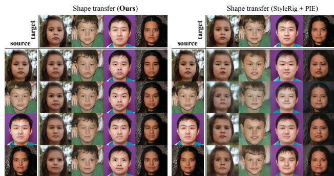
Figure 5: Shape transfer comparison. We transfer the 3D shape of each source image to each target image while keeping everything else unchanged. Our results ( left ) demonstrate more accurate shape transfer and much better disentanglement between shape and other attributes (e.g., albedo, pose, and hair) than the combination of StyleRig (Tewari et al. 2020a) and PIE (Tewari et al. 2020b) ( right ).
