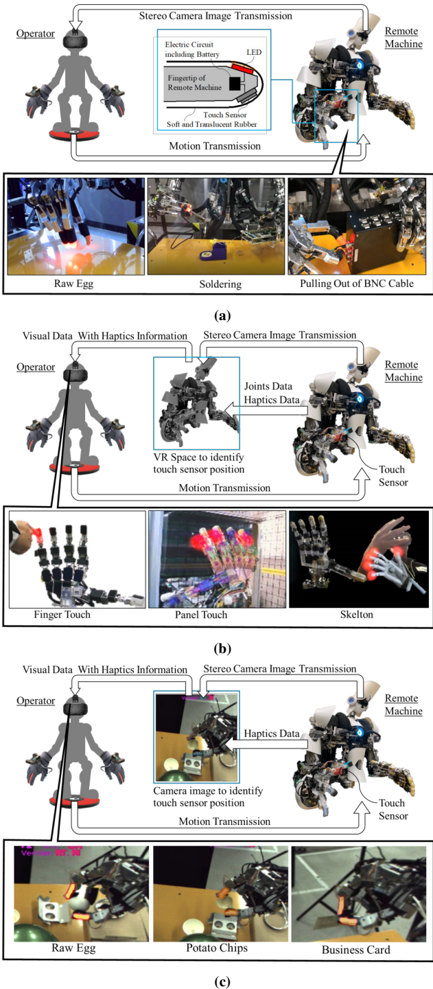
Fig. 12: Prototype implementation of visual haptics: (a) base verification with an LED mounted on the fingertip; (b) superimposition on the robot model; (c) dexterous manipulation with superimposed images based on color tracking.
