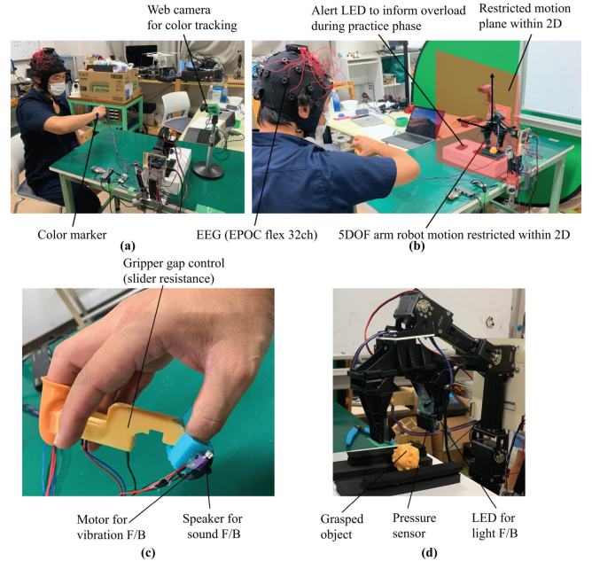
Fig. 2: Evaluation equipment for three feedback modalities: (a, b) experimental scenes; (c) gripper gap controller with vibration and sound feedbacks; (d) robot arm with light feedback.
