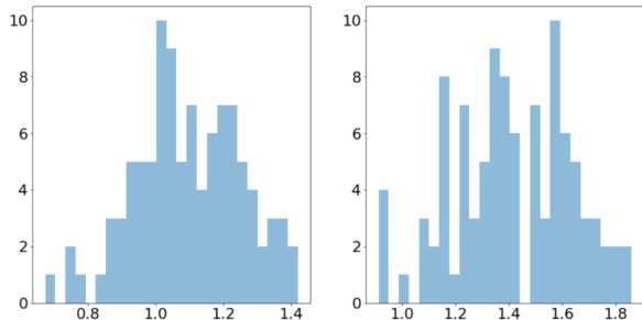
Fig. 7: Proposed model performance histogram for individual comfort models. X-axis (left) MAE [ ^{\circ}\text{C} ] (right) RMSE [ ^{\circ}\text{C} ]
