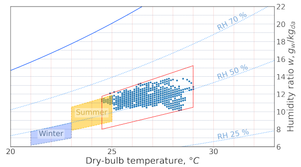
Fig. 1: Possible methods of specifying thermal comfort zones on the psychrometric chart.
