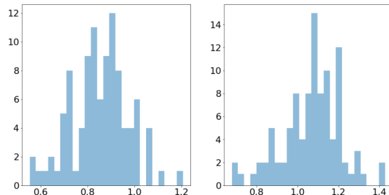
Fig. 8: Proposed model performance histogram for combined comfort models. X-axis (left) MAE [ ^{\circ}\text{C} ] (right) RMSE [ ^{\circ}\text{C} ]
