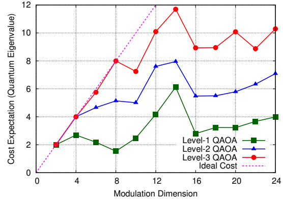
Fig. 5: Expected cost function with optimized variational angles as a function of dimension.
