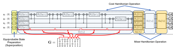
Fig. 2: Quantum gate diagram of QAOA demodulation.
