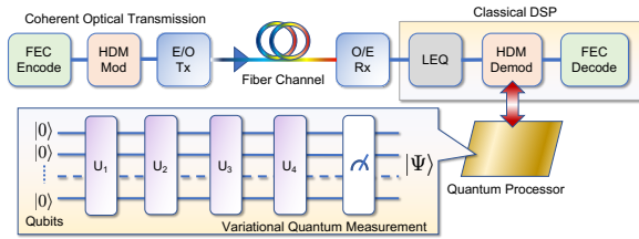
Fig. 1: QPU-assisted coherent optical transmission.
