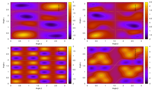
Fig. 4: Landscape of cost expectation for level-1 QAOA demodulation of 4, 6, 8, and 12-D modulations.
