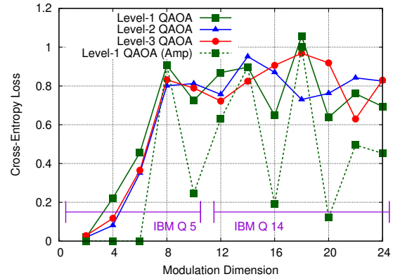
Fig. 7: Cross-entropy loss on real QPUs with variational angles optimized via ideal simulations.
