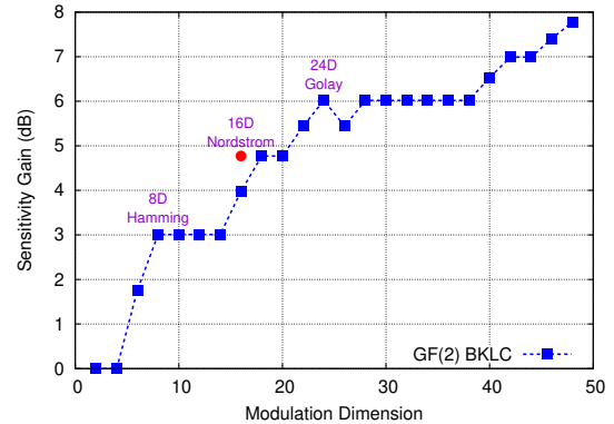
Fig. 3: Sensitivity gain of block-coded HDMs over 1-D BPSK as a function of modulation dimension.
