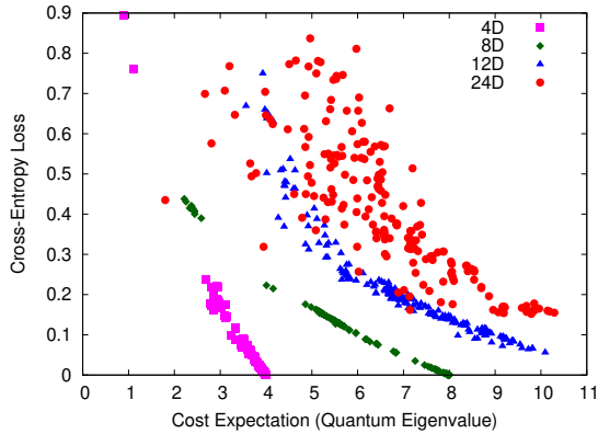
Fig. 6: Variational factor optimization for level-3 QAOA demodulation of 4, 8, 12, and 24-D HDMs.
