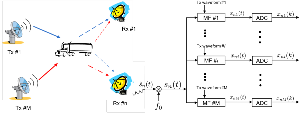
Fig. 1. Moving target detection of distributed MIMO radar and baseband signal at local receivers.
