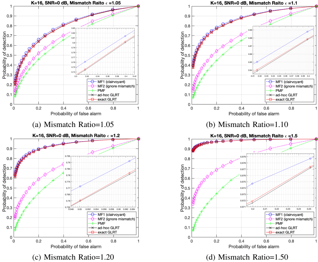
Fig. 5. ROC (receiver operating characteristic) curves for various local detectors as a function of mismatch ratio when SNR = 0 dB. MF1: the optimal matched filter with the knowledge of target residual; MF2: matched filter ignoring the target residual; PMF: projection matched filter; Ad hoc: an ad hoc GLRT of [44]; GLRT: proposed GLRT.
