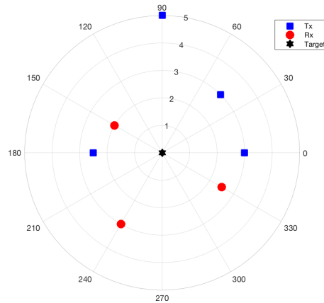
Fig. 7. The distributed MIMO radar configuration considered in simulation.
