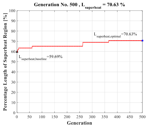
Figure 3. IPGA optimization progress
