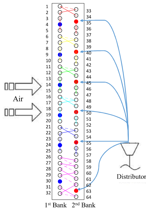
Figure 4. Optimal heat exchanger circuitry
