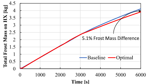
Figure 7. Frost mass transients
