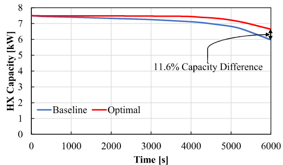
Figure 6. Evaporator capacity transients
