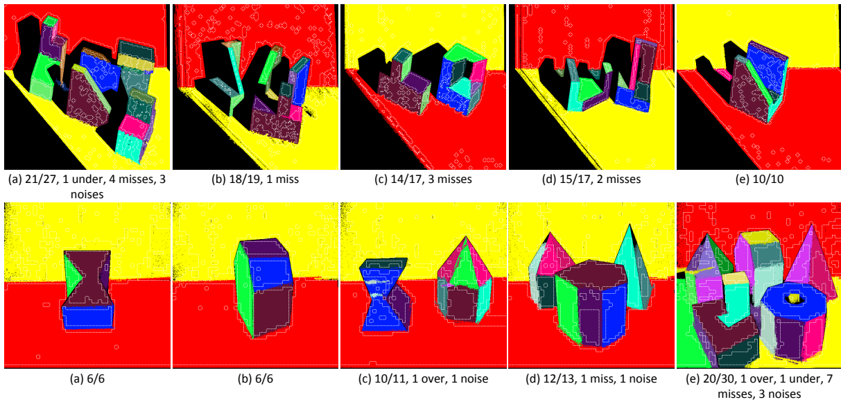
Fig. 9. Plane extraction on SegComp datasets. The estimated plane normal deviated from the ground truth was (1.7 \pm 0.1)^\circ for ABW-TEST (top) and (2.4 \pm 1.2)^\circ for PERCEPTOR-TEST (bottom). Again, white dash lines are the segmentation boundary before the region-grow-based refinement.
