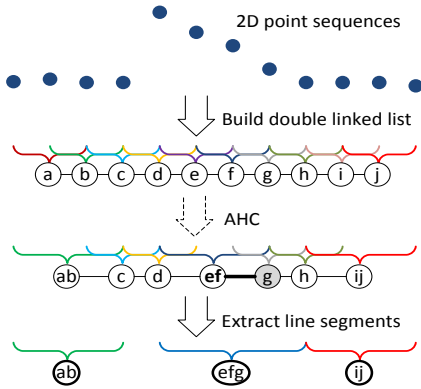
Fig. 3. Line regression algorithm. Blue dots show the 2D points. Circles labeled with letters show the nodes in a linked list. Brackets show the groups of points represented by the nodes. Thick line indicates that merging node g with its left neighbor ef gives a smaller line fitting MSE than merging it with its right neighbor h .
