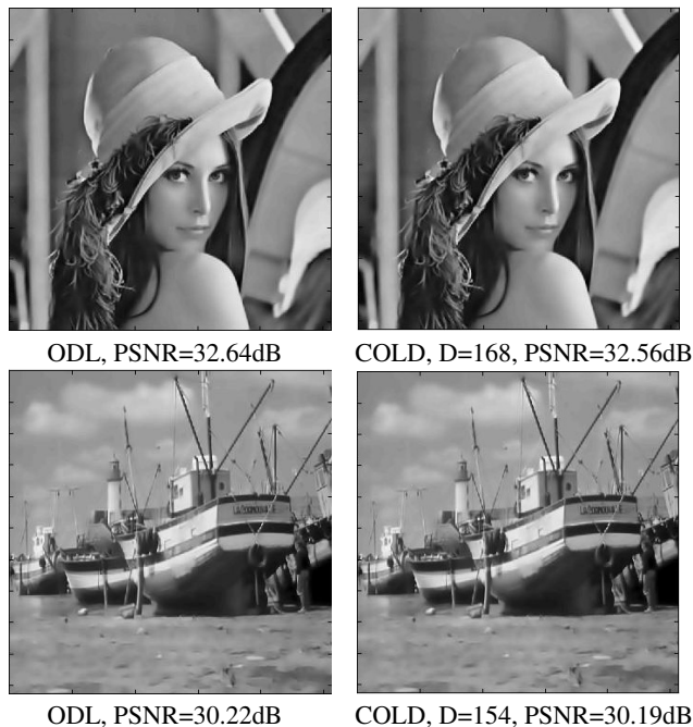
Fig. 5. Images on the left are the reconstruction obtained from ODL and the one on the right is the reconstruction using COLD. D denotes the dictionary size.
