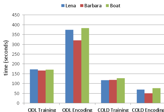
Fig. 6. Reconstruction times taken by ODL and COLD.
