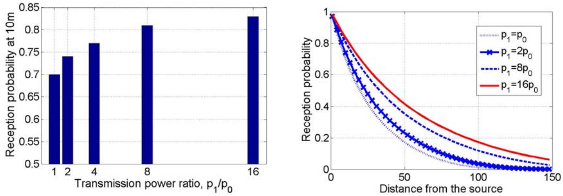
Figure 2 (left) Reception probability of a specific source at 10 m, and (right) Reception probability as a function of distance. The transmit power of background traffic is p_0 = 27 dBm, the transmit power of the specific source is p_1 , c=0.05 , \lambda=0.25 veh/m, BPSK.
