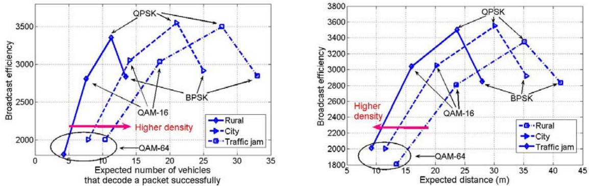
Figure 7 Tradeoff of broadcast efficiency and reliability due to modulation scheme.
