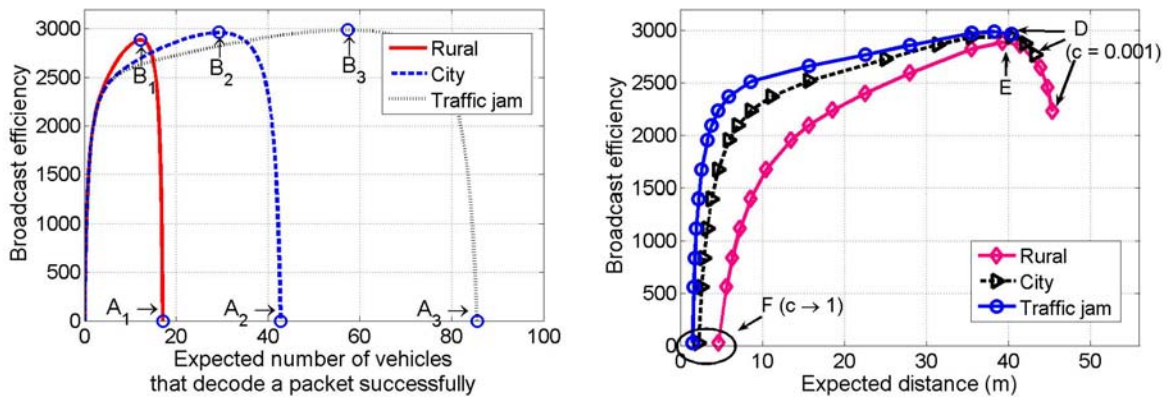
Figure 6 Tradeoff of broadcast efficiency and reliability due to transmission probability: (left) broadcast efficiency vs. expected number of vehicles that decode a packet successfully, and (right) broadcast efficiency vs. expected distance. p_0=27 dBm, L=512 bits, BPSK.
