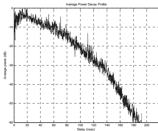
Figure 2 Average power delay profile for CM 3
