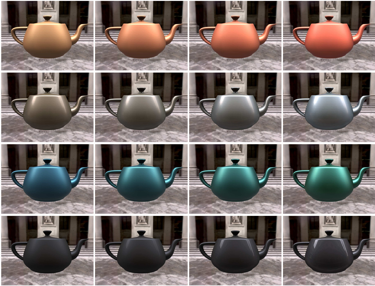
Figure 15: Navigation in the linear space. Each row corresponds to changing one parameter of the model. The first row shows an increase in the redness trait applied to the GoldPaint BRDF. The second row illustrates an increase in the silverness trait applied to the SpecularGold BRDF. Row three applies the gold-like trait to the BlueGlossyPaint BRDF. The fourth row shows an increase in the specularness trait applied to the BlackMattePlastic BRDF.
